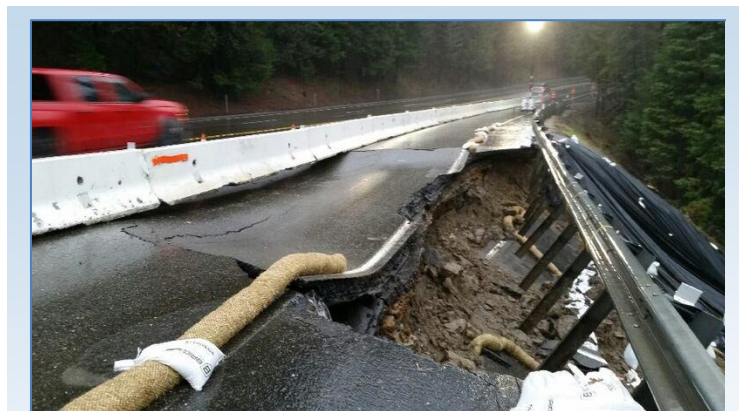
Severe Erosion on U.S Highway 50 in 2017
