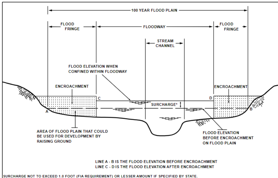
Figure 4-27 Floodplain Schematic
